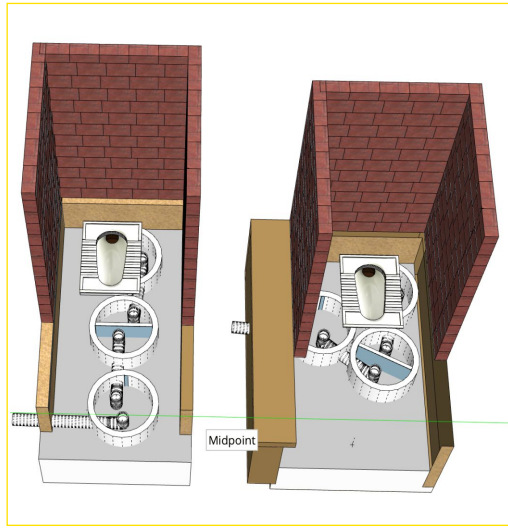
Getting septic tanks through narrow lanes at beneficiary doorstep
