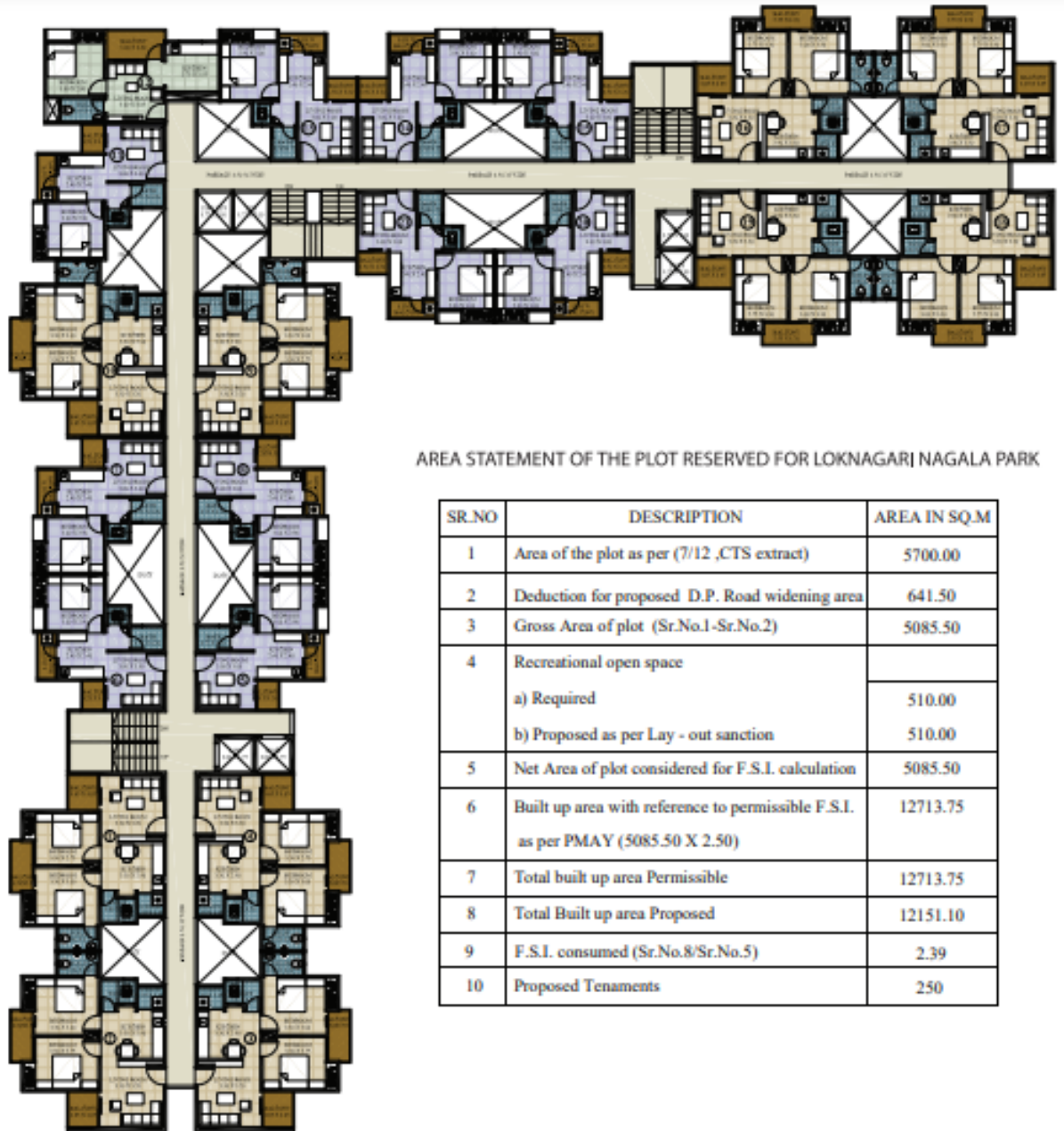
Figure. 4.8 Loknagari floor layout
